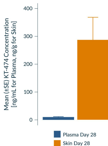
High KT-474 Exposure in HS and AD Patients Skin
