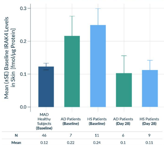
Reduced IRAK4 in Skin Lesions of AD and HS Patients
